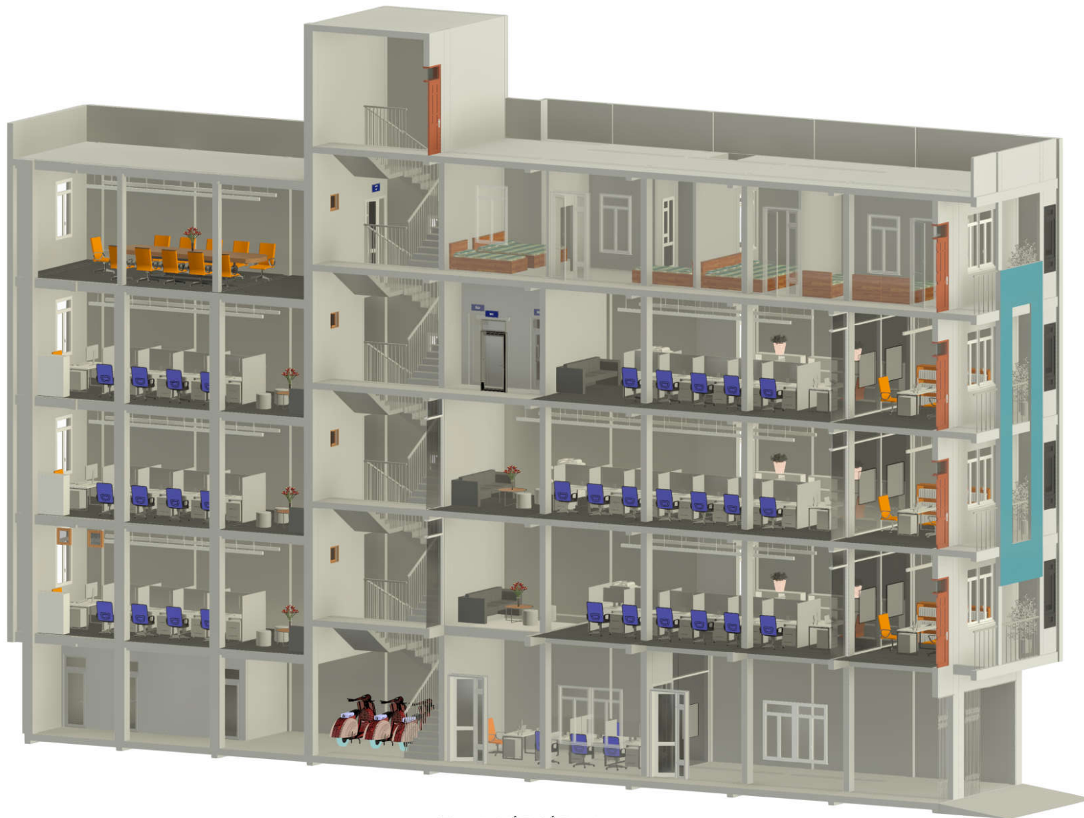
KC-11 1 TL 3D MẶT CẮT 1-1
